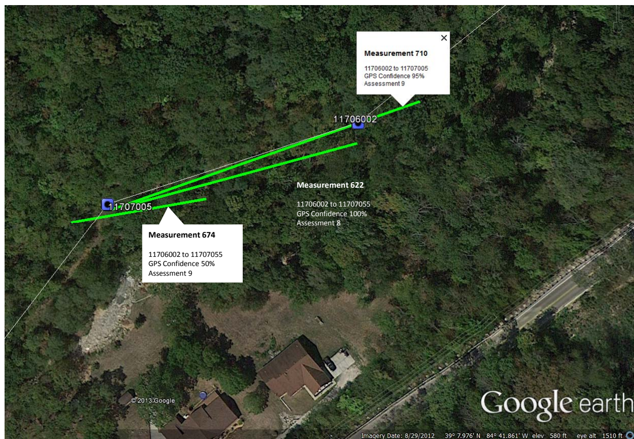
Figure A-2. GPS mapping for the three SL-RAT condition assessments conducted at Galia road pipe segment 11706002-11707005.
